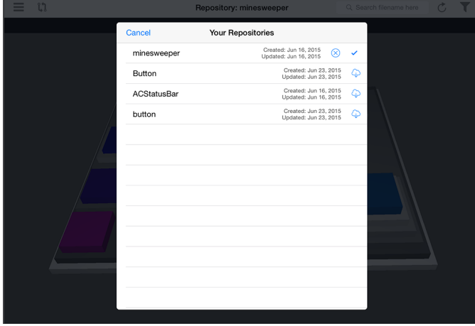
Fig. 2. Repository List
